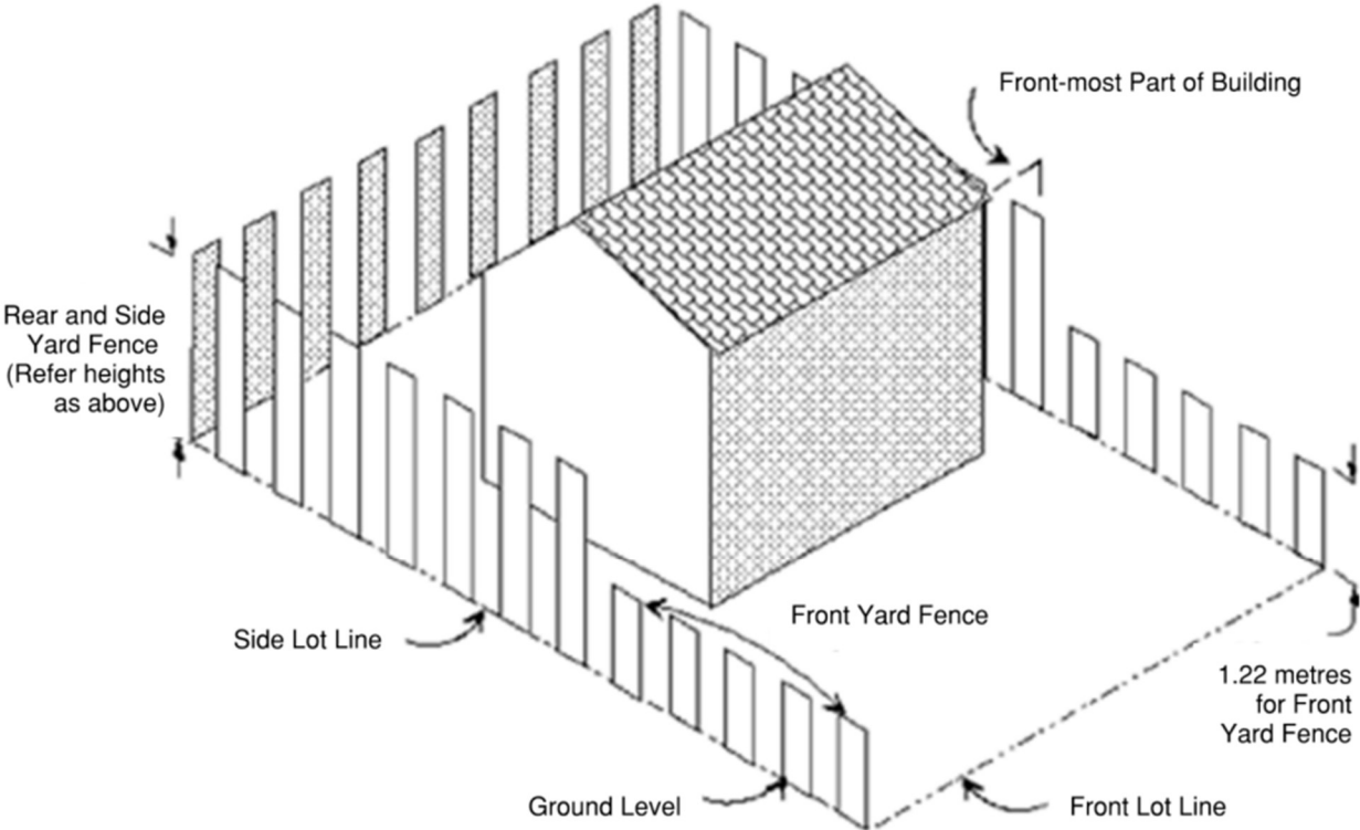
Figure 2D.F3: Fencing Requirements
